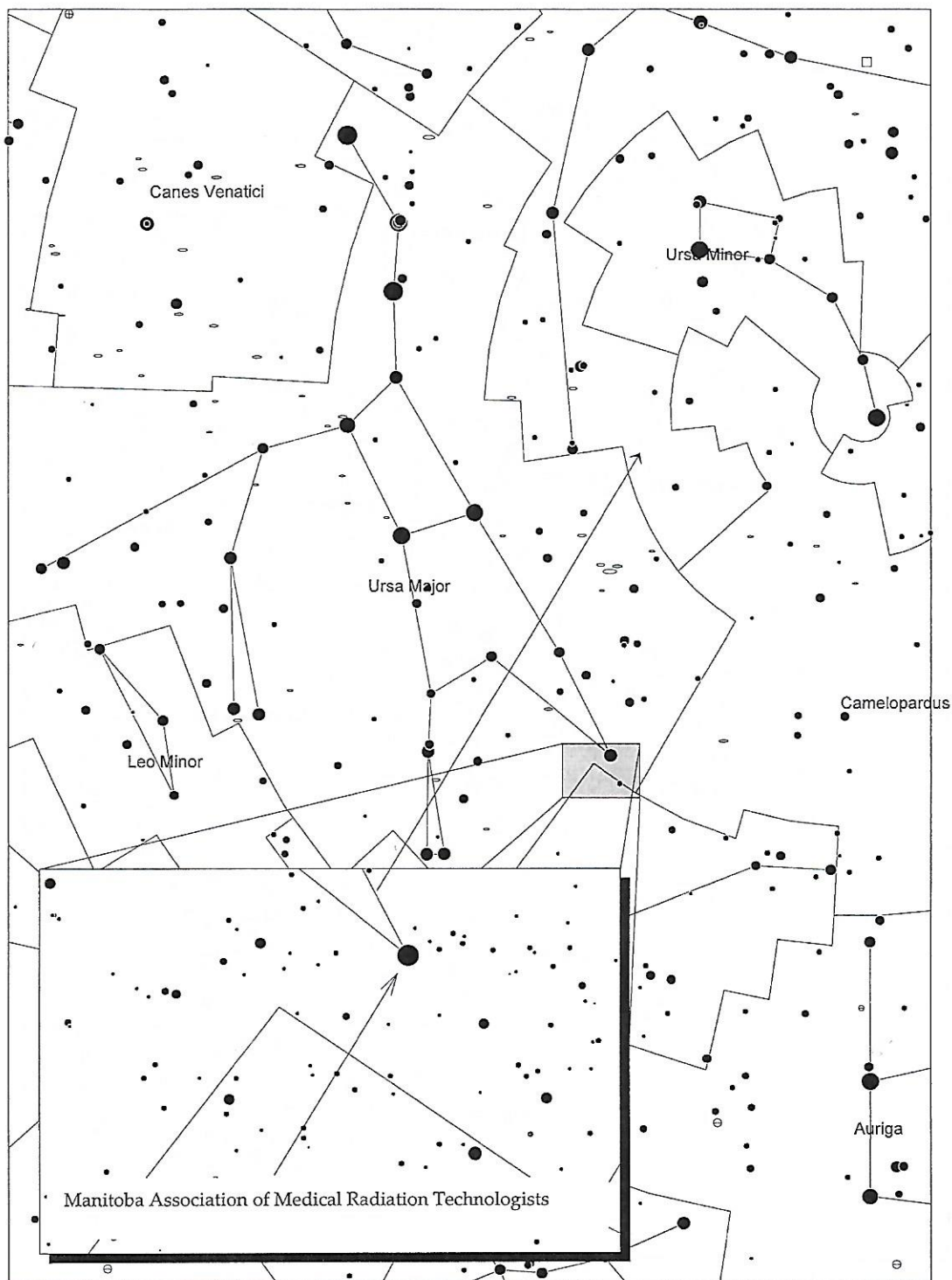
Star finder chart for SAO 14573 in Ursa Major
