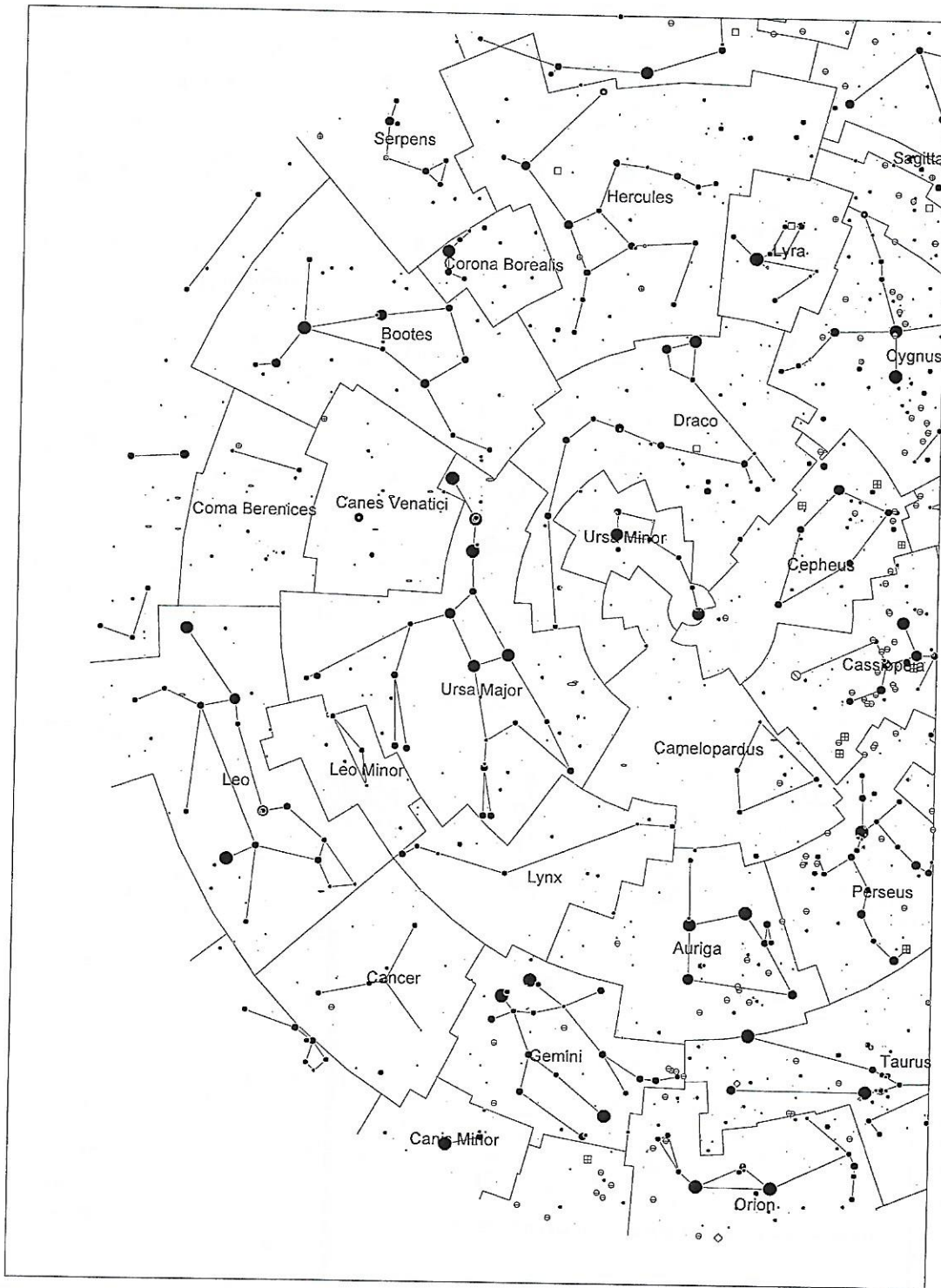
Constellation finder chart for Ursa Major .
